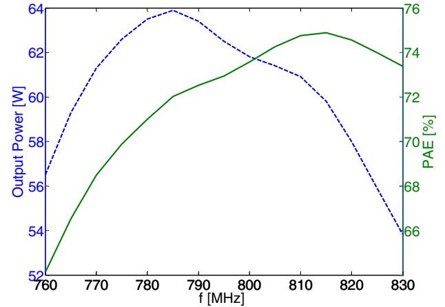
Fig. 3. Measured (--) output power (left) and (-) PAE (right) vs. frequency at an input power level of 25dBm.
