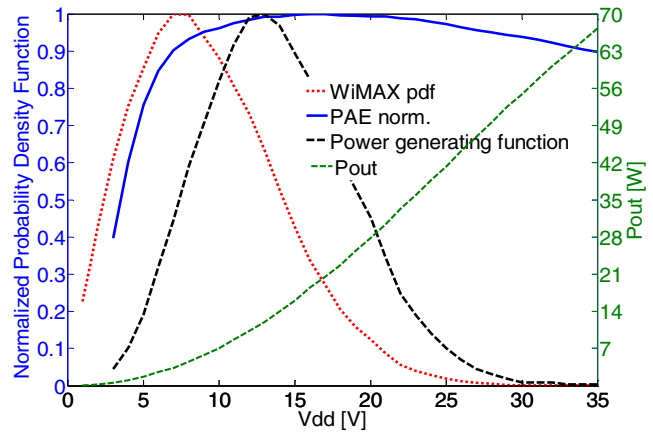
Fig. 4. Amplitude component pdf for a WiMAX signal, P_{out} , power generating function [1], and normalized PAE (to a maximum value of 79%) vs. V_{dd} .
