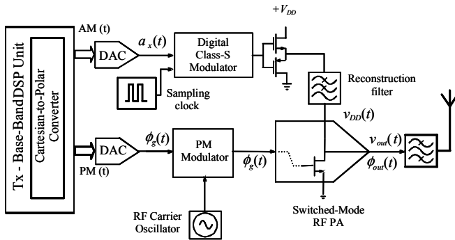
Fig. 1. System level representation of a wireless polar transmitter
