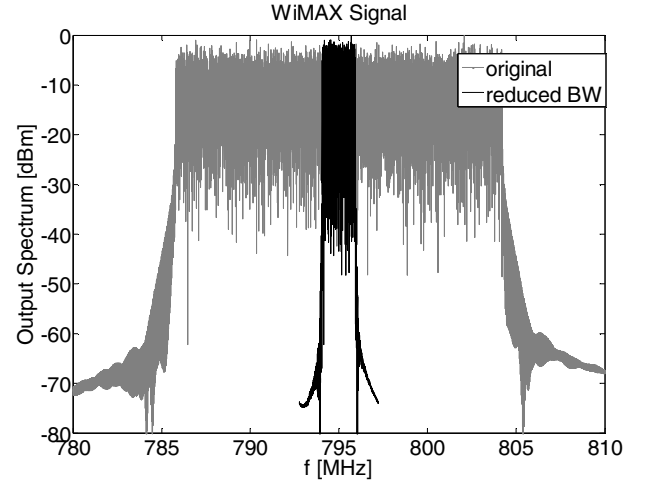
Fig. 7. 20 MHz (original) and 2 MHz (software reduced) bandwidth WiMAX signal spectra.
