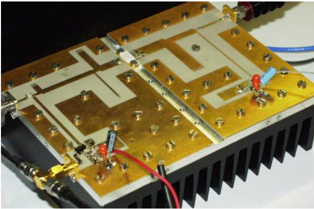
Fig. 2. Photograph of the implemented PA.
