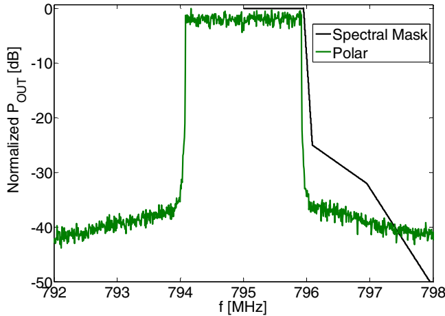
Fig. 8. Normalized output spectrum.
