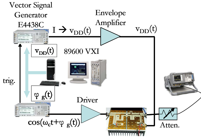
Fig. 6. Polar transmitter test set-up.
