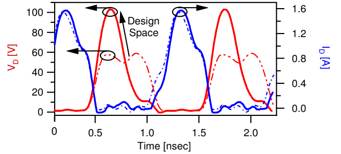
Fig. 2. Simulated current and voltage waveforms at the Igen-plane for a 10W GaN HEMT device for the standard Class-F mode (dotted lines) and “Continuous Class-F” mode (solid lines) for \gamma=-1 .
