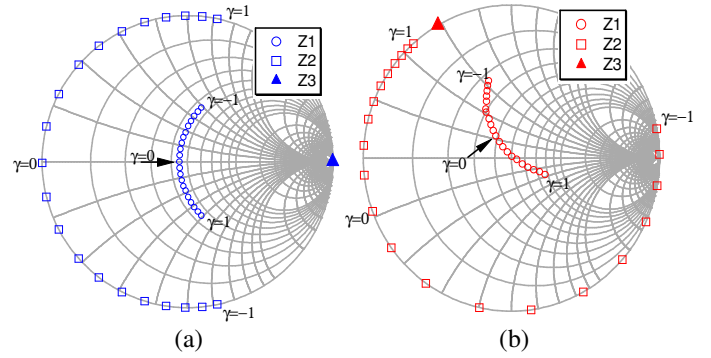
Fig. 1. First three harmonic target impedances for the 10W GaN HEMT device at the Igen-plane (a) and at the device-package measurement plane (b).
