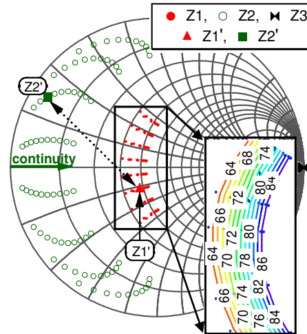
Fig. 5. Extended continuous class-F mode with second harmonic impedance inside the Smith chart with \beta = \alpha/1.9 when varying \alpha between 0.6 and 1.5 and \gamma between -0.7 and 0.7, inset efficiency contour for fundamental load points.
