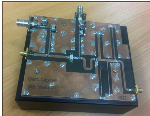
Fig. 7. Realized Continuous Class-F 10W power amplifier.
