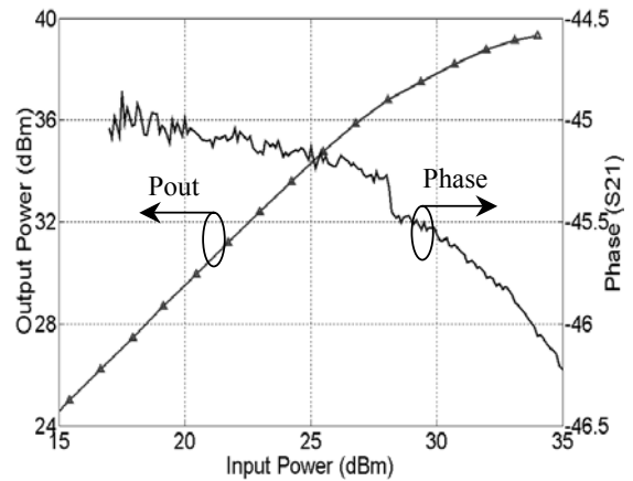
Fig. 12 AM/AM and AM/PM measurements at F = 1 GHz, V_{DS} = 30 V and I_{DS} = 500 mA.
