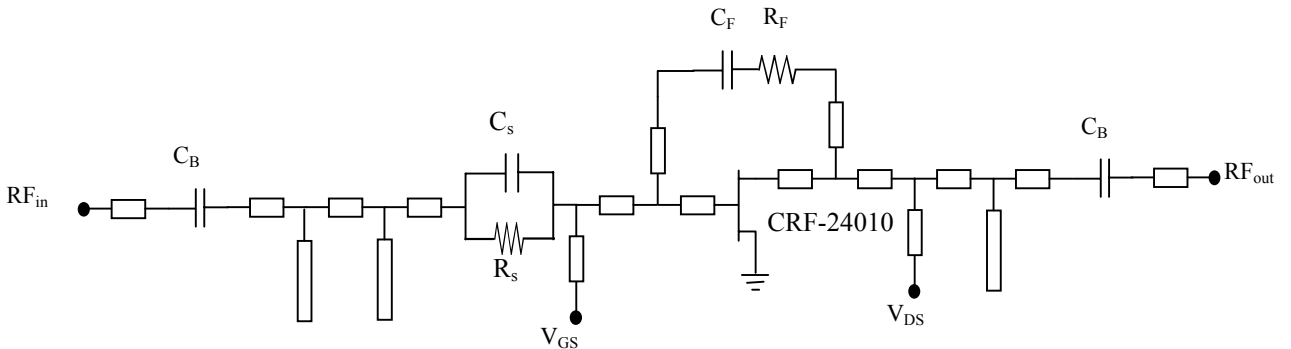
Fig. 3. Schematic diagram of broadband 5 W power amplifier.
