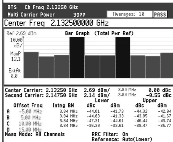
Figure 8. W-CDMA Result at 6W Average Output
