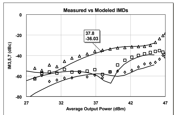
Figure 7. Intermodulation Results
