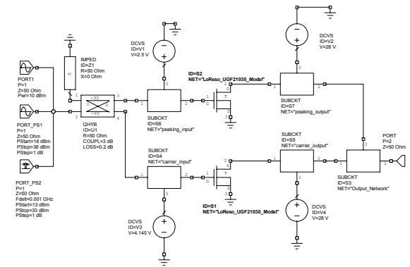
Figure 3. Complete Doherty Amplifier Model
