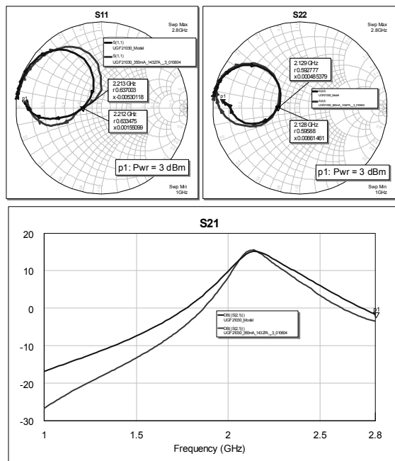
Figure 1. Fits to s-parameter data for UGF21030
