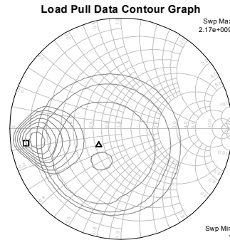
Figure 2. Fits to load and source pull data for UGF21030
