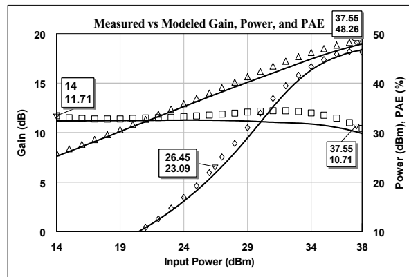
Figure 6. Large Signal Power Sweep
