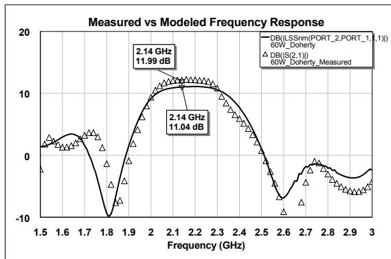
Figure 5. Small Signal Results
