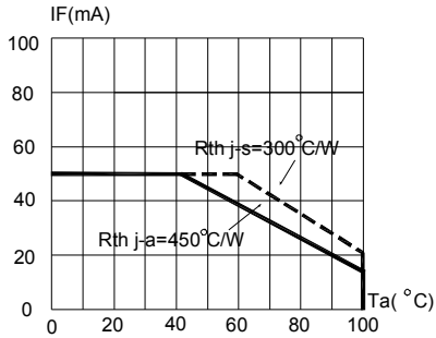
FIG.5 MAXIMUM FORWARD DCCURRENT VS AMBIENT TEMPERATURE (Tjmax=110°C)
