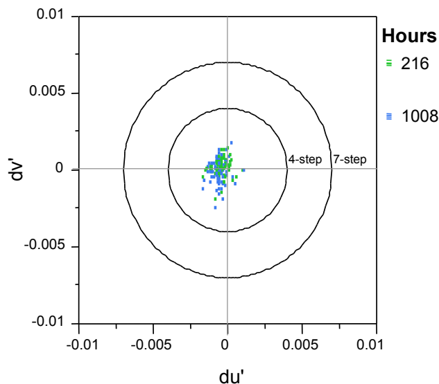
XLamp MC-E Warm White LED - White Point Stability: I_F = 700 \text{ mA} @ 85^\circ\text{C} (3500 K)
